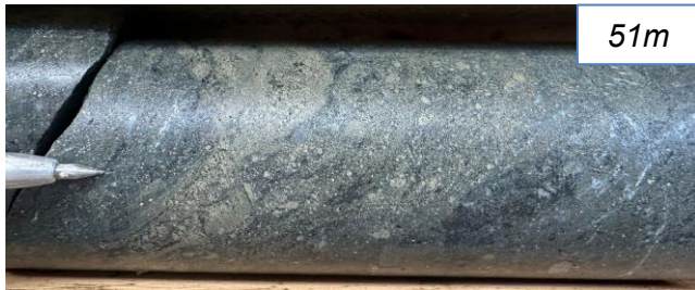
Sulfide flooded domain in chlorite altered andesite fragmental: 0.085 g/t Au 410 ppm Cu / 3m (48-51m)
