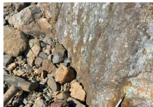
VMS Zone massive sulfide 3.73% Cu, 6.46% Zn, 0.447 g/t Au, 58.2 g/t Ag
