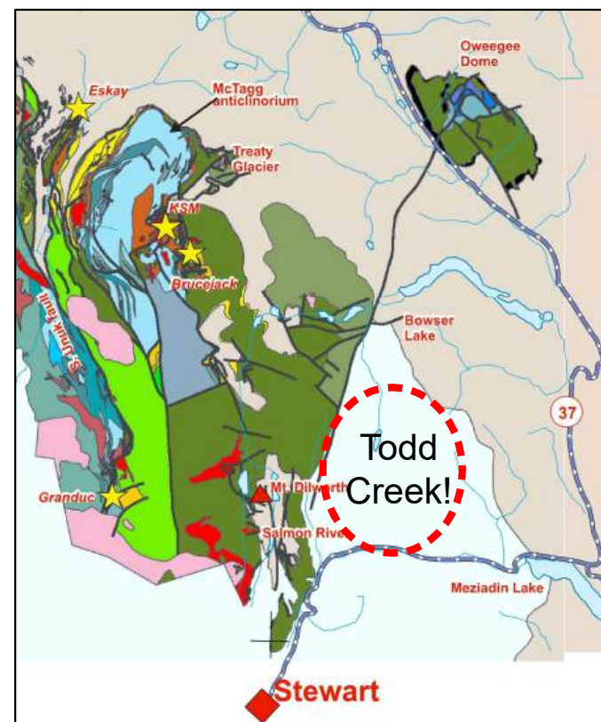
Map of Hazelton Group, Nelson et al., BCGS Paper 2018-1.
