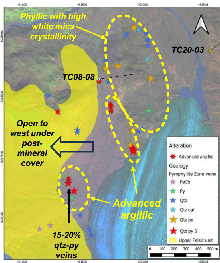
Pyrophyllite Zone showing vein and alteration types, upper felsic unit, and drill holes
