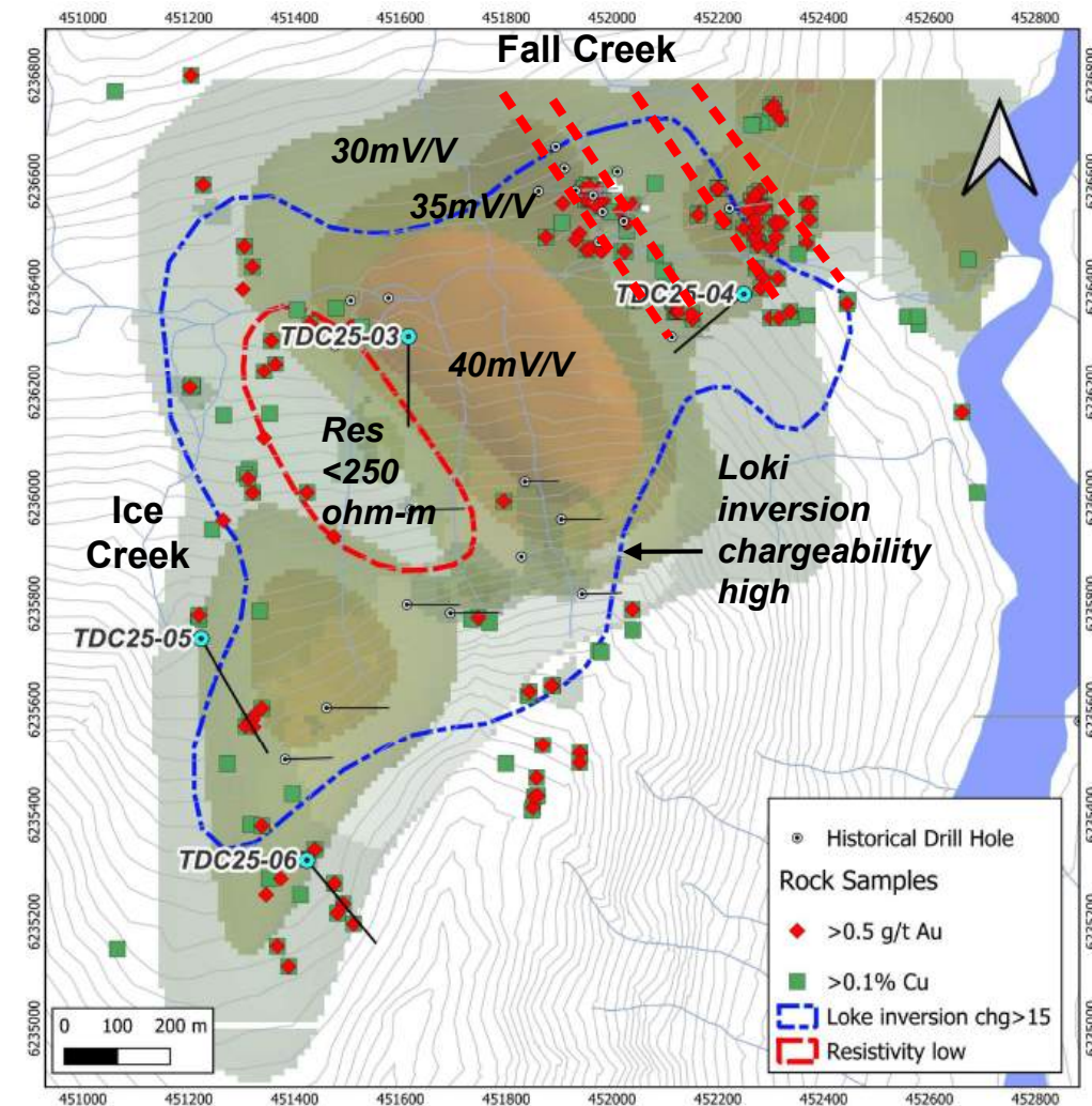
IP anomalies, DH collars and rock samples with Cu > 0.1% or Au > 0.5 g/t
